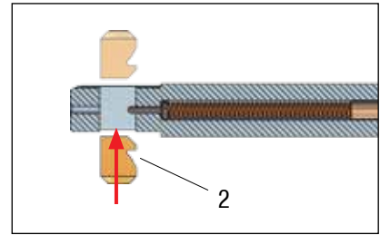
The deburring blade is pushed with its back into the blade window of the tool until it engages. Please make sure that it is aligned with the recess (2) in the direction of the tool shank. The blade can be inserted into the tool from both sides.
