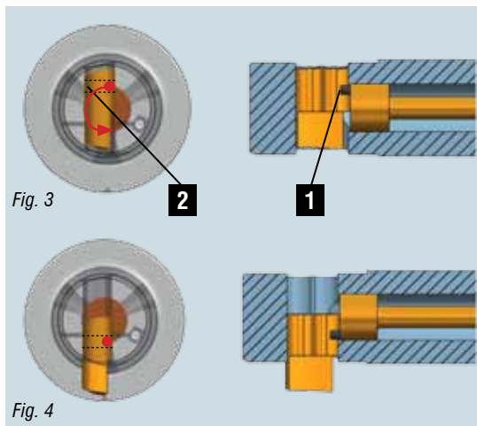
1: Control Pin 2: Blade Slot Fig. 3: Blade retracted Fig. 4: Blade extended
